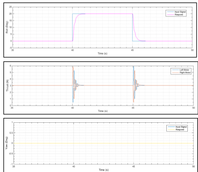
Figure 19 Rolling without Main Rotor Tilt.
